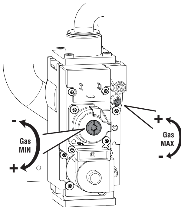
Valvola gas FUTURA 3 F
